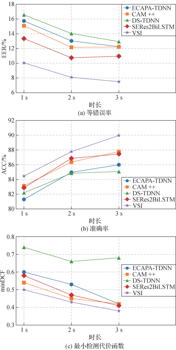
图7 不同时长下模型指标对比实验结果 Fig. 7 Experimental results under different durations (a) EER; (b) ACC; (c) minDCF
