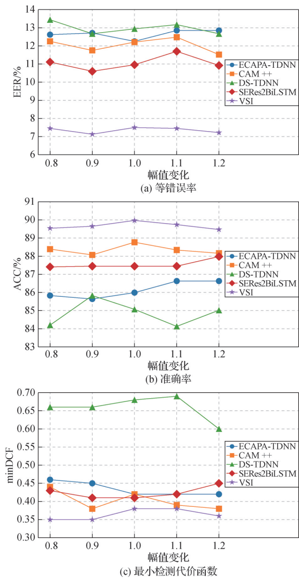
图 10 不同幅值下模型指标对比实验结果 Fig. 10 Experimental results of model under different amplitude variations ((a) EER; (b) ACC; (c) minDCF)
