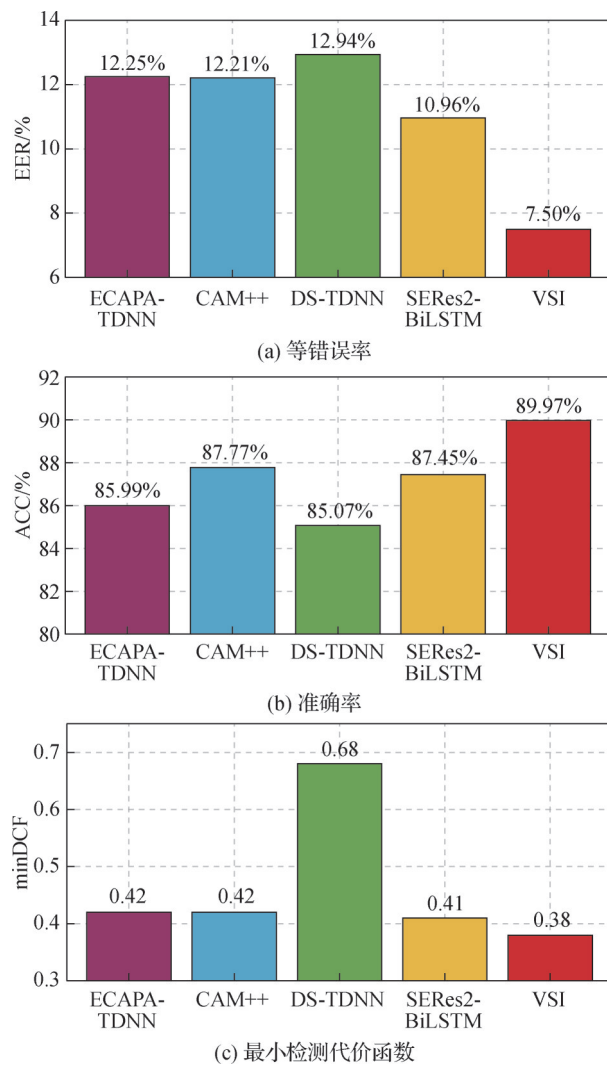
图5 5种模型的对比实验结果 Fig. 5 Comparative results of five models (a) EER; (b) ACC; (c) minDCF
