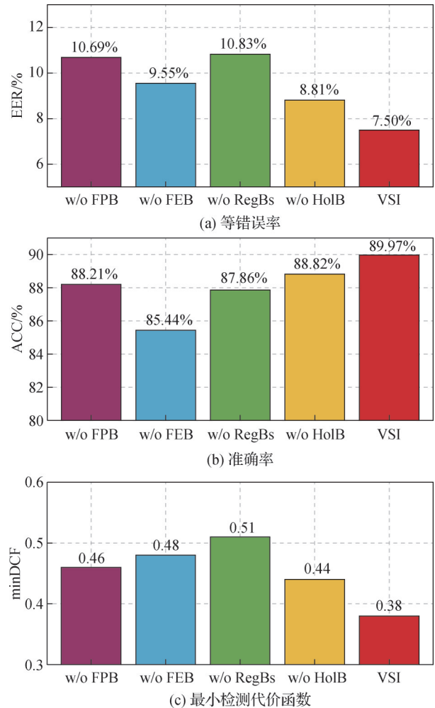
图6 VSI模块有效性实验结果 Fig. 6 Validation results of the VSI blocks (a) EER; (b) ACC; (c) minDCF
